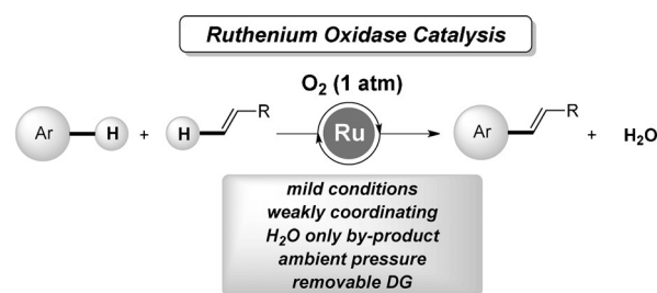
Figure 1. Ruthenium oxidase catalysis for C–H alkenylations.
