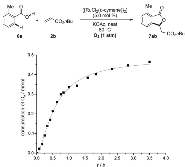
Figure 2. Oxygen consumption during ruthenium(II)-catalyzed C–H activation.
