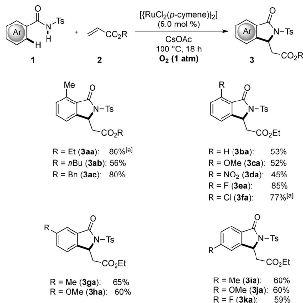
Scheme 1. Aerobic ruthenium(II)-catalyzed assembly of isoindolinones 3 . [a] KOAc instead of CsOAc.
