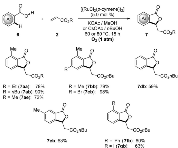
Scheme 3. Aerobic ruthenium(II)-catalyzed synthesis of phthalides 7 .
