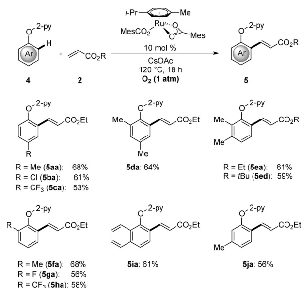
Scheme 2. Oxidase catalysis for C–H alkenylation with a removable DG. py = pyridyl; Mes = mesityl.
