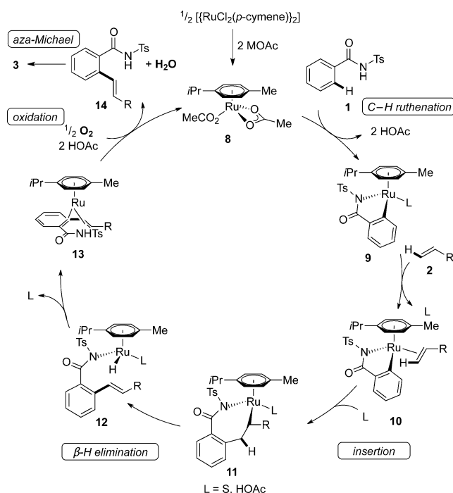
Scheme 4. Proposed catalytic cycle for ruthenium oxidase C–H alkenylation. L = ligand.
